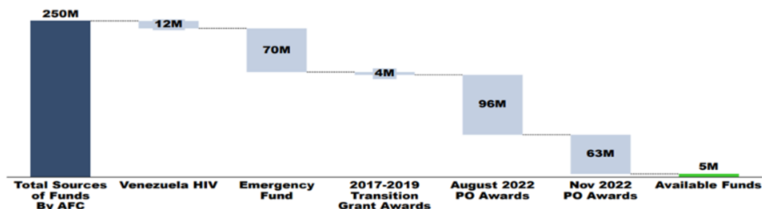
Figure 7. 2020-2022 Portfolio Optimization
